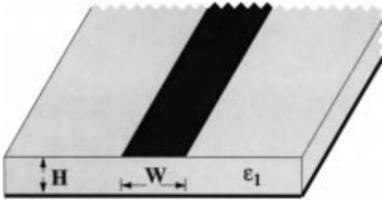
Fig. 1. Cross section of an open microstrip line.
